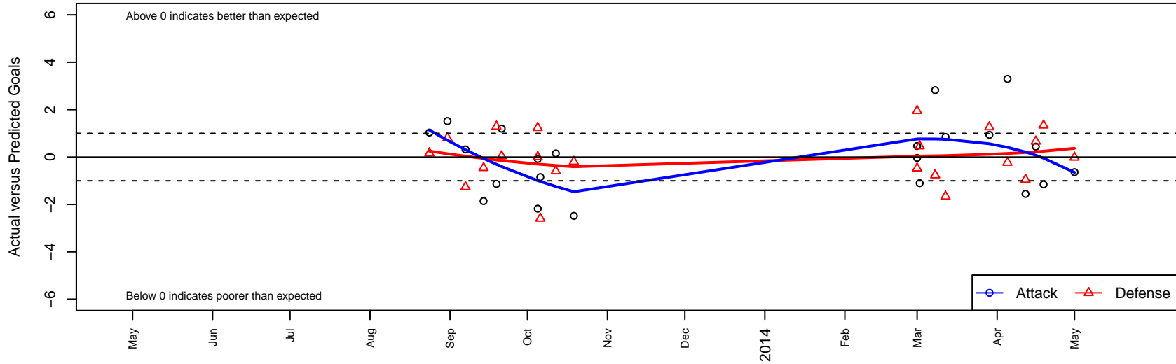
FC Nova Grey G01 Dots are actual minus expected GF (blue circles) and GA (red triangles). Blue line is smoothed change in attack strength. Red is smoothed change in defense strength.
